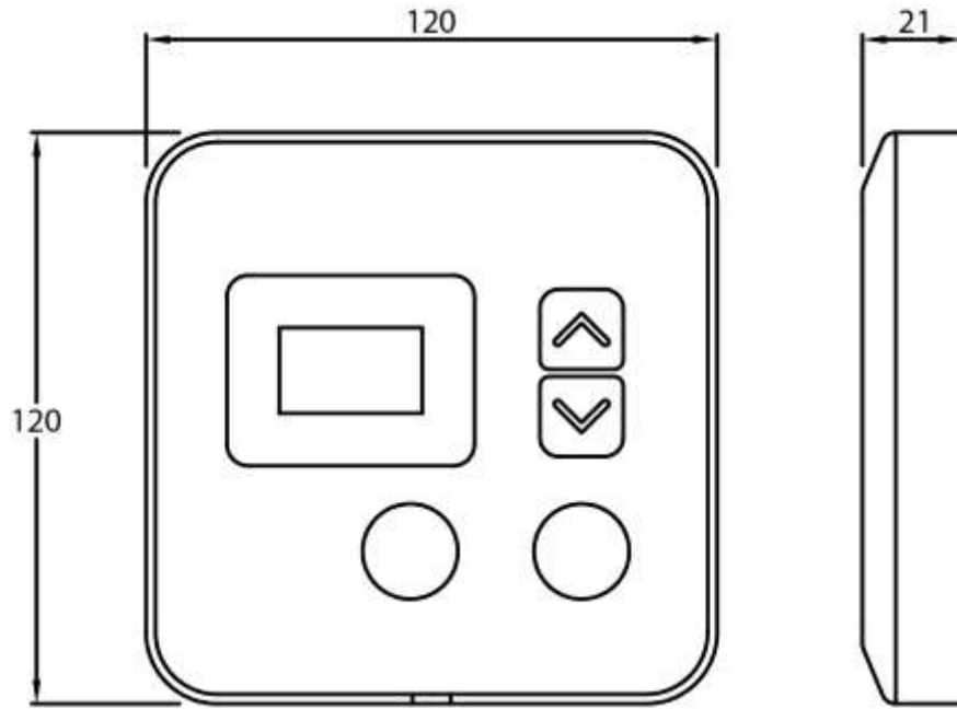
Kitchen Controller
