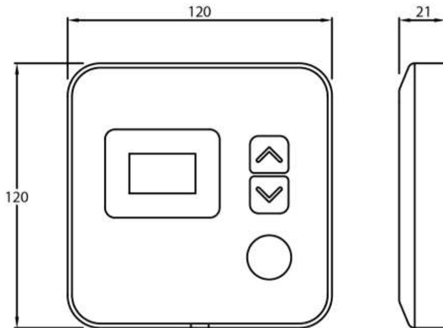
Bathroom Controller
