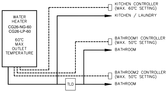
CG26-60 series
