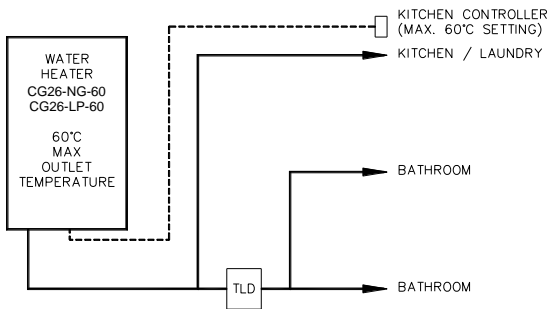
CG26-60 series
