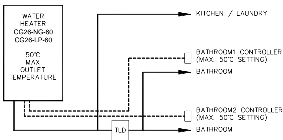
CG26-60 series
